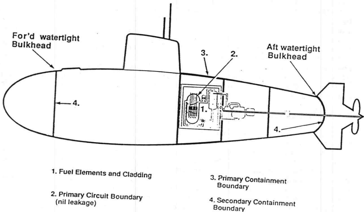
FIG 2.1 - BARRIERS TO FISSION PRODUCT RELEASE
